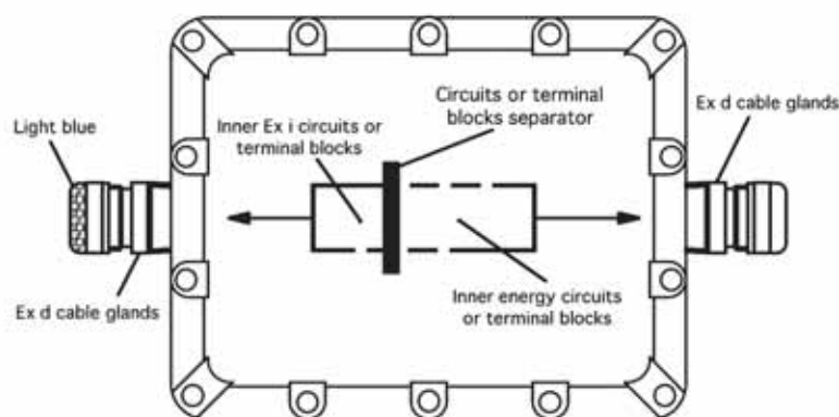
1) Ex d Junction box
