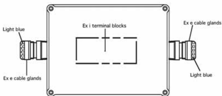
3) Ex e Junction box painted light blu
